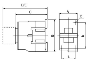
CJX2-D09-32
